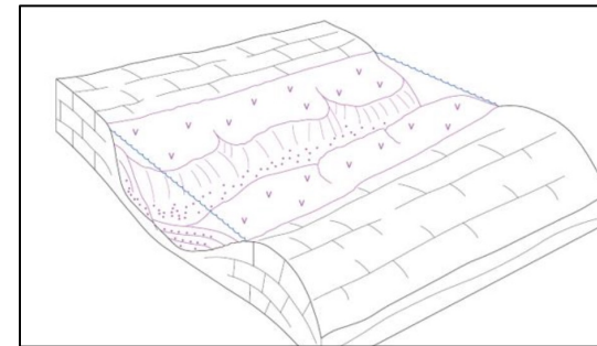
Deep water subaqueous evaporites in intrashelf basin
