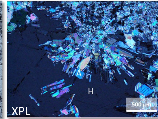
Anhydrite rosettes cemented by halite
