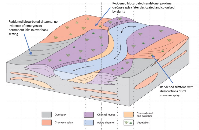
Facies model of Ugle Fm
